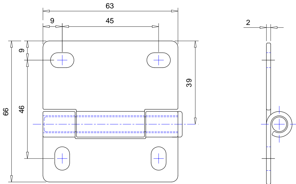
Typical hinge dimensions
